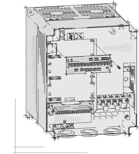
Mounting an option card to the FR-A 540 EC
